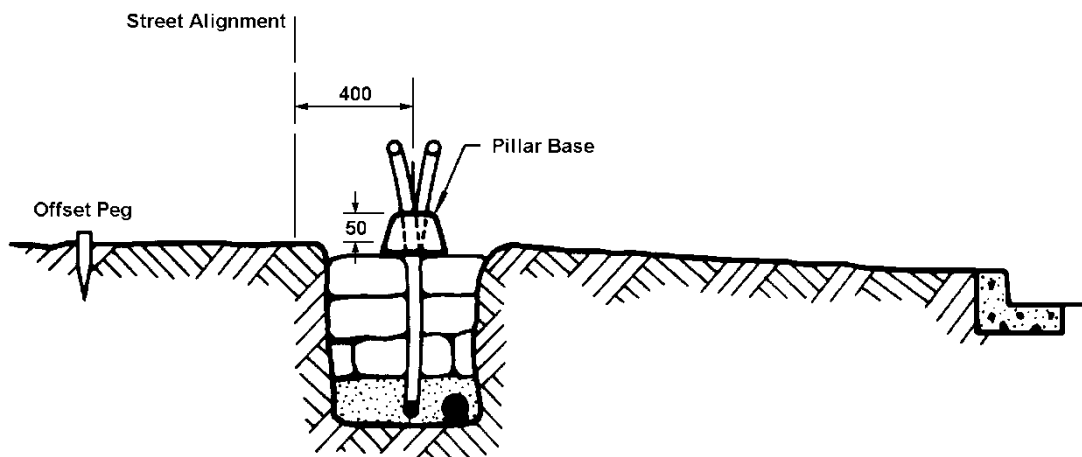
Figure 14: Pillar Base Alignment Details
