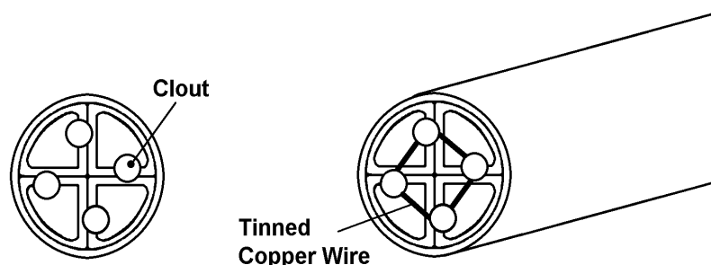
Figure 18: Shorting the cable
