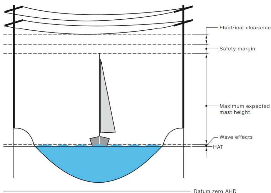
Figure 17 – Clearances for Navigable Waterway crossings
