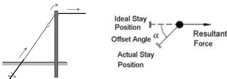
Figure 5 - Stay Loading and Offsetting
