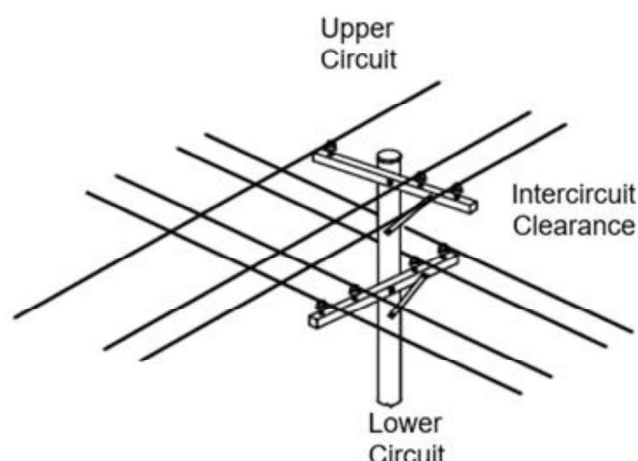
Figure 13 - Conductor Clearances for Different Circuits on the Same Support
