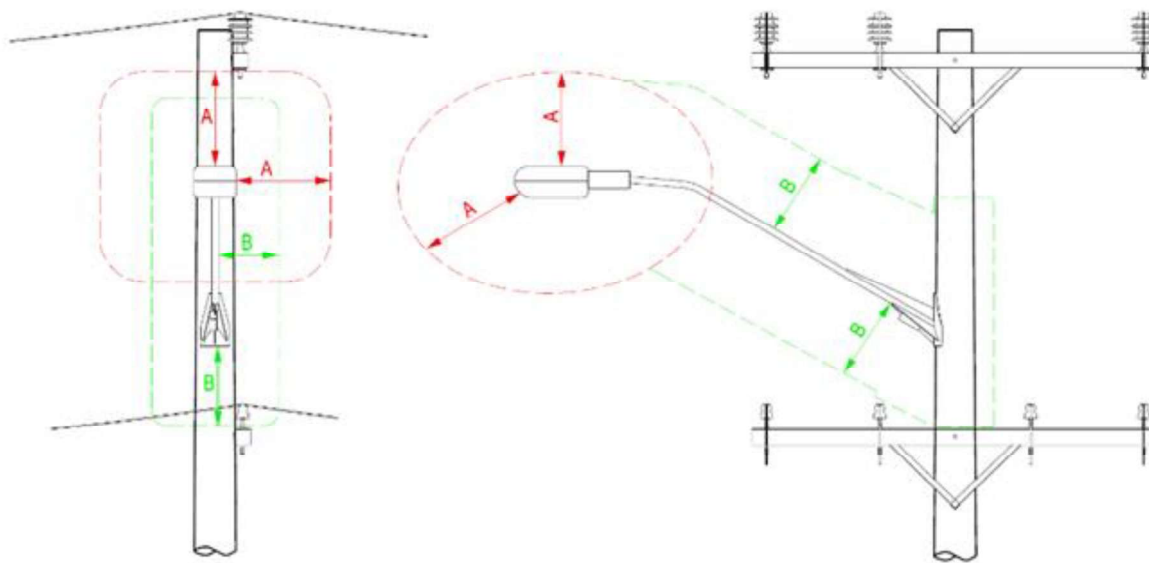
Figure 19 – Clearances to Streetlights Attached to the Same Pole
