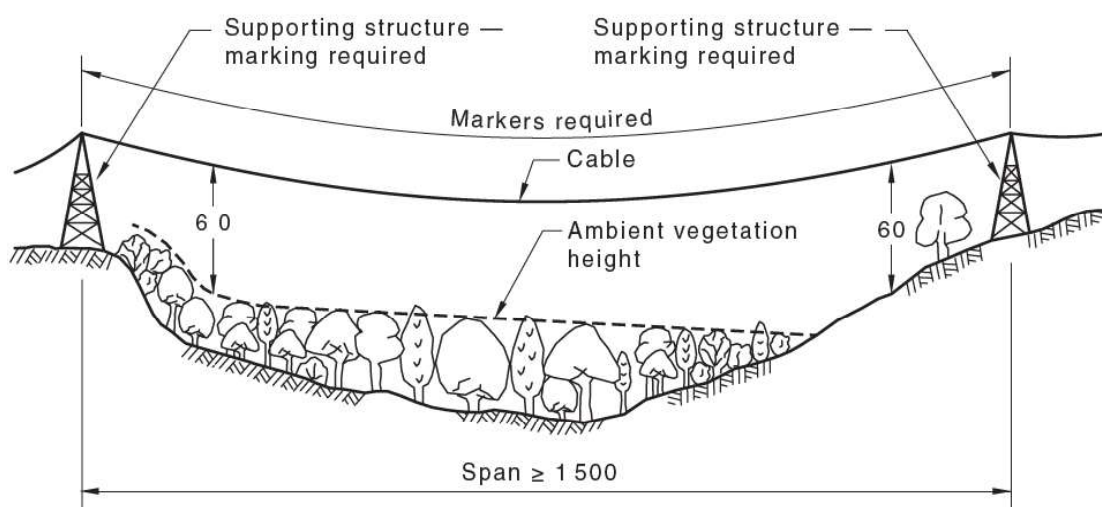
Figure 23 – Span greater than 1500m long and 60m high (Source AS3891.1)
