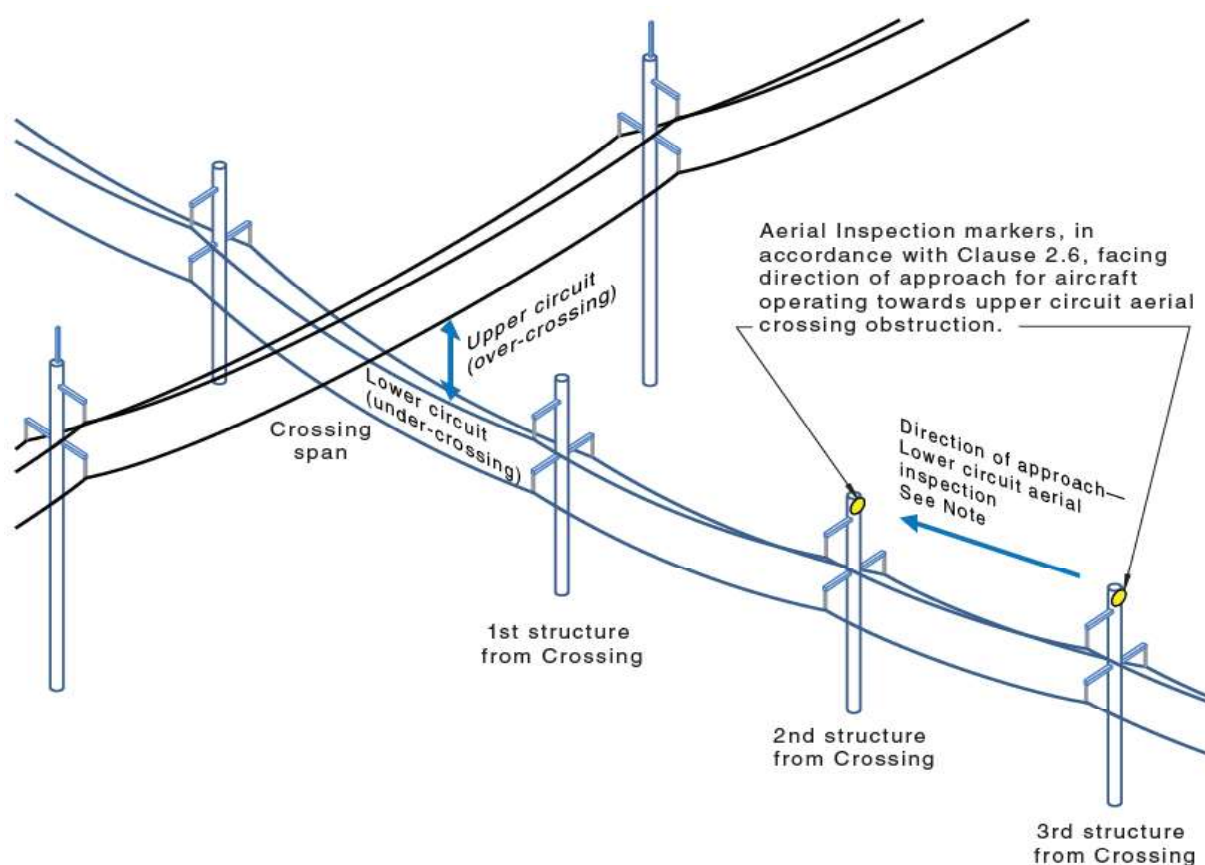
Figure 24 – Aerial warning marker placement for low level operations (Source AS3891.2)
