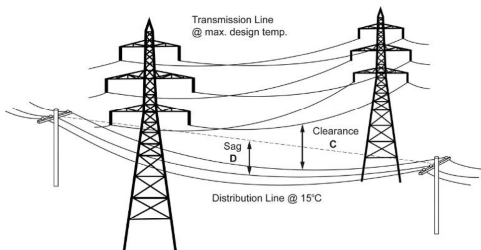
Figure 16 – Clearances for Transmission Under-crossings
