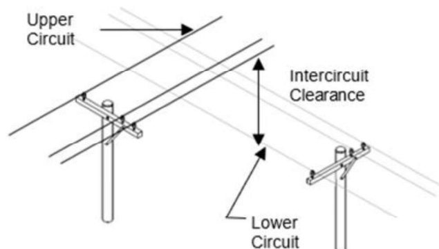
Figure 14 – Conductor Clearances for Unattached Crossings
