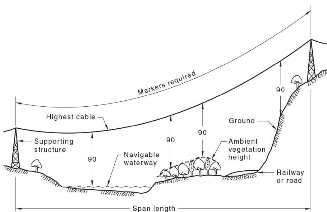
Figure 22 – Span height greater than 90m (Source AS3891.1)
