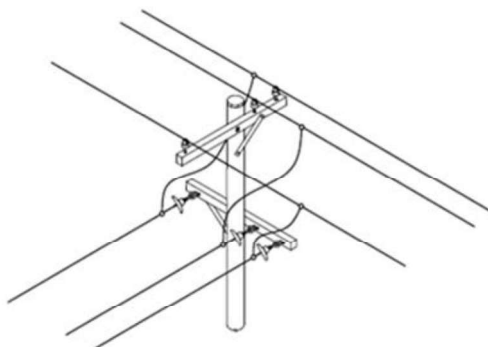
Figure 12 - Conductor Clearances for the Same Circuit on the Same Support
