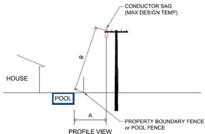
Figure 20 – Clearances to Swimming Pools and Pool Surrounds
