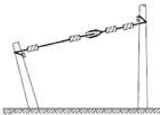
Figure 8 – Aerial (Pole) Stay Arrangement
