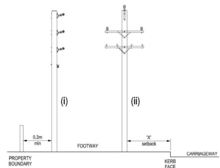
Figure 4 - Pole Alignment / Setback Options
