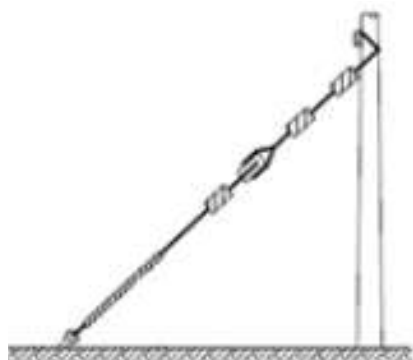
Figure 6 – Ground Stay Arrangement
