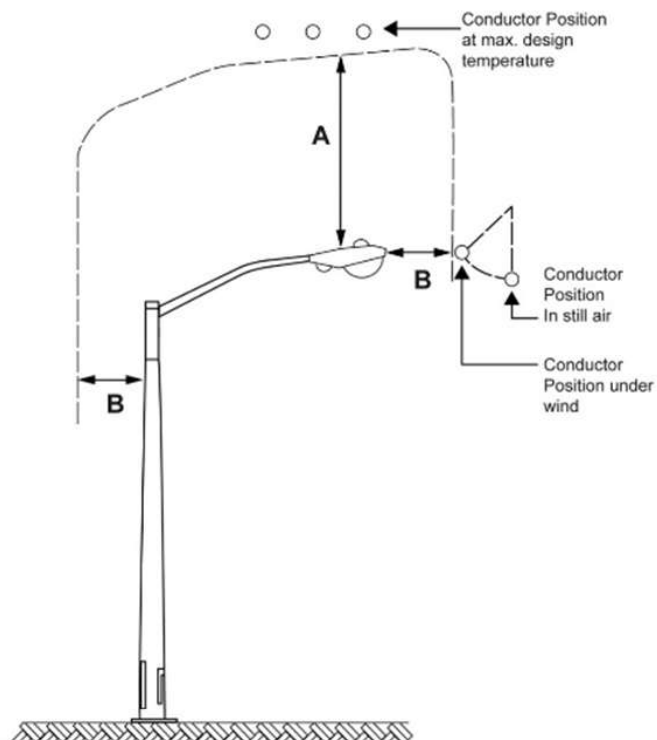
Figure 18 – Clearances to Streetlights Not Attached to the Same Pole
