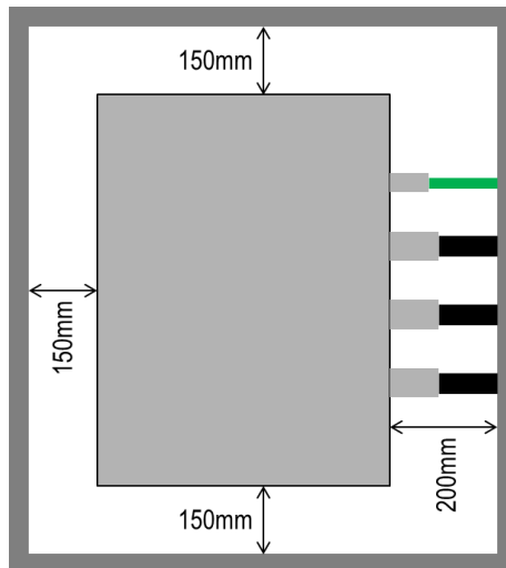
Figure 2 - minimum clearance between link box and link box pit
