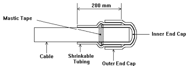
Figure 10 - Sealed cable
