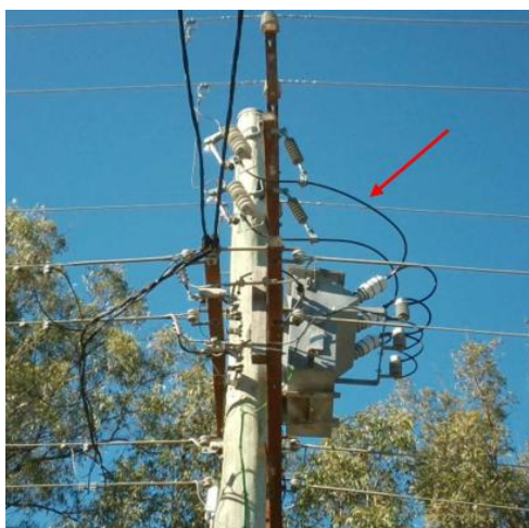
Figure 50 – An example of an 11kV unscreened cable that must be treated as exposed
