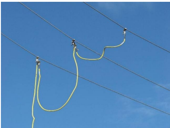
Figure 58 - Three phases earthed and short-circuited on HV overhead line
