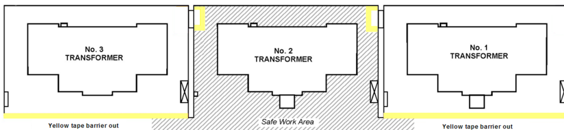
Figure 35 - A diagram illustrating barrier-out method used on transformer bays
