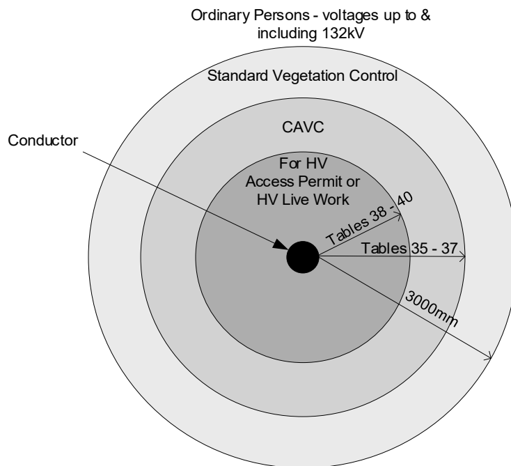
Figure 60 - Vegetation clearance from energised overhead mains
