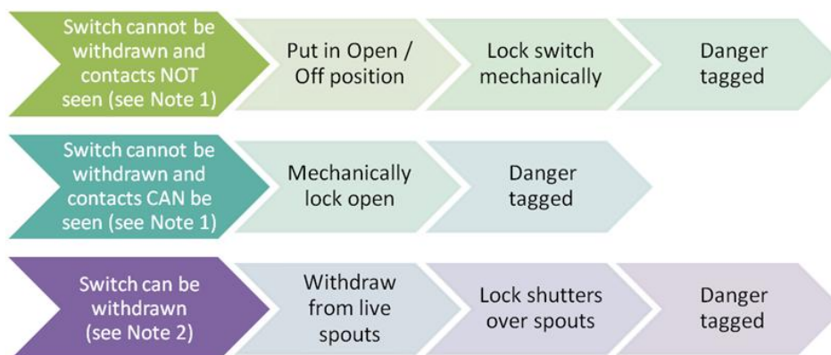
Figure 54 - Precautions taken when operating a switch to isolate high voltage mains and apparatus.
