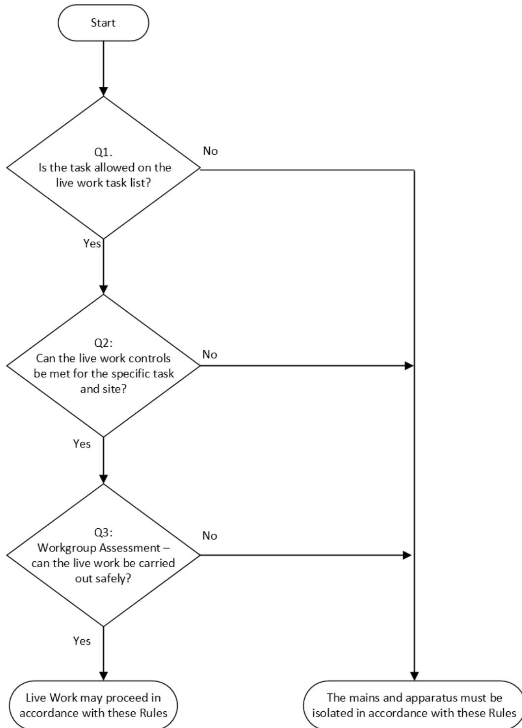
Figure 52 – Flowchart illustrating the LV work planning process
