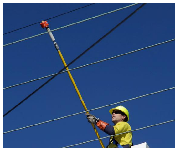
Figure 57 - Proving HV conductors are de-energised
