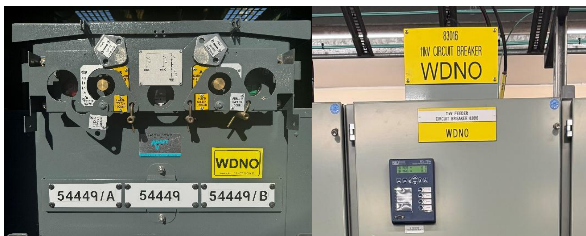
Figure 36 – Examples of switches labelled WDNO
