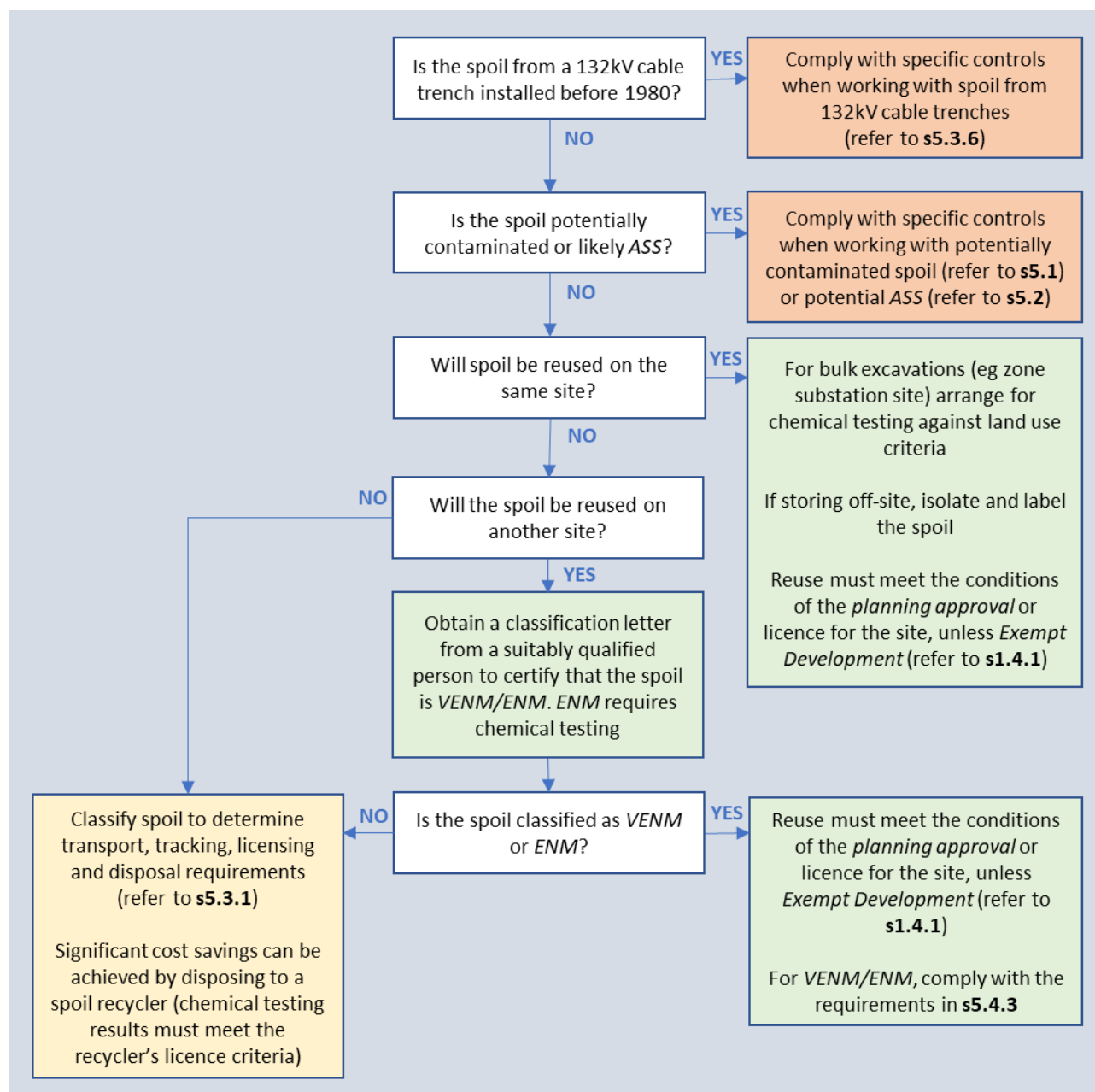
Figure 5.3-2: Process for managing spoil
