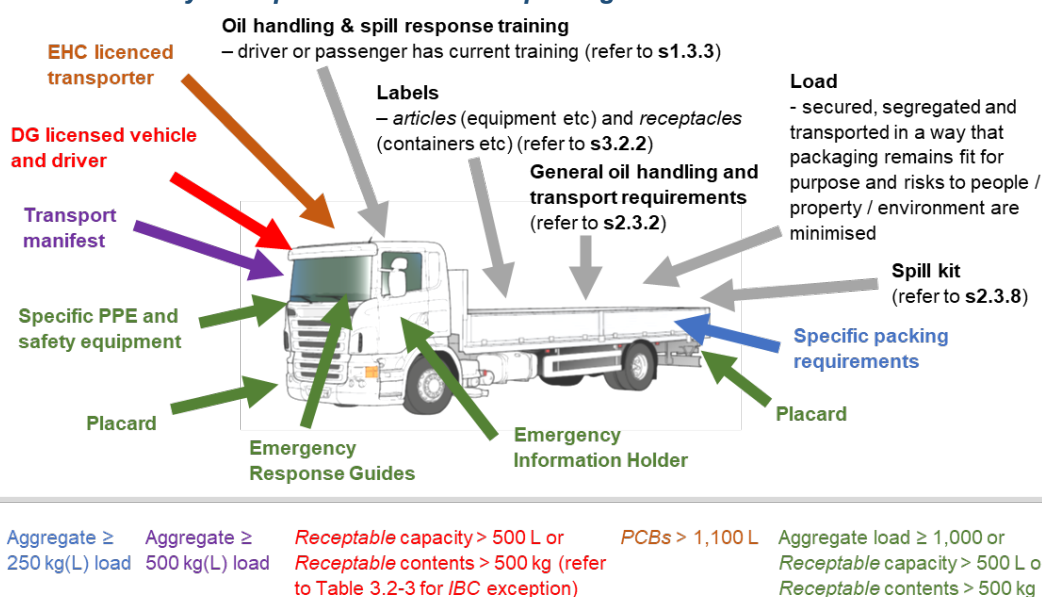
Figure 3.2-2: Summary of requirements for transporting scheduled PCB
